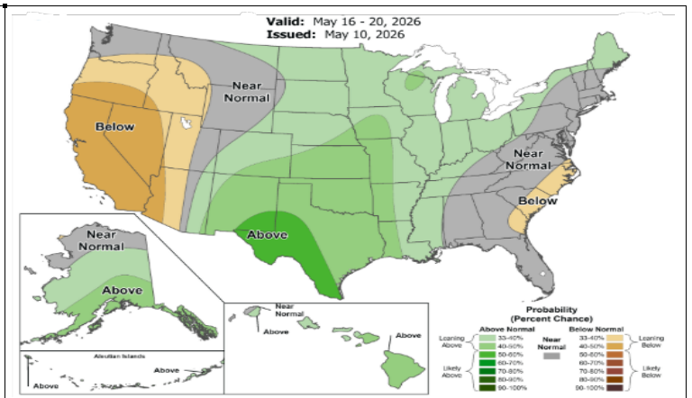
Precipitation
