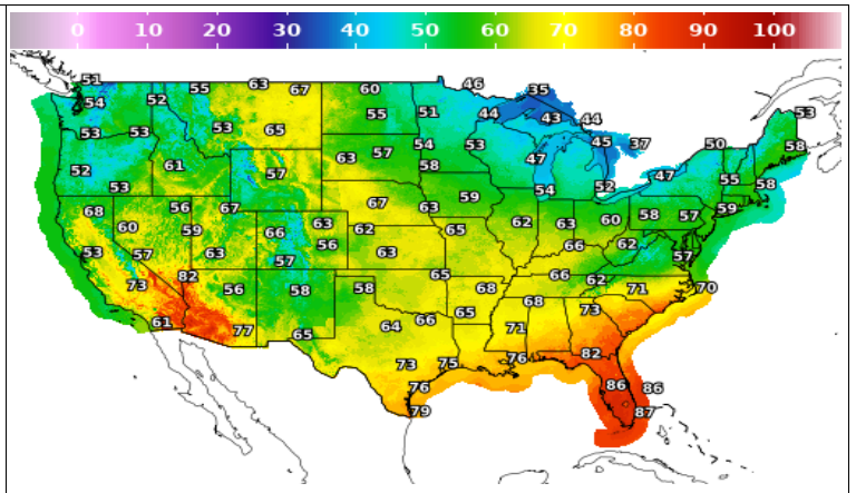
LOW Temperature
