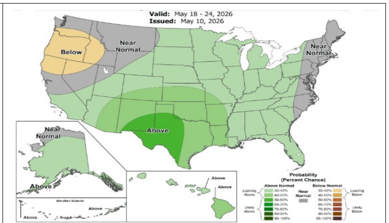
Precipitation
