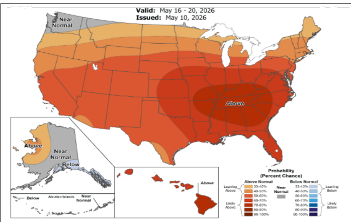
Temperature
