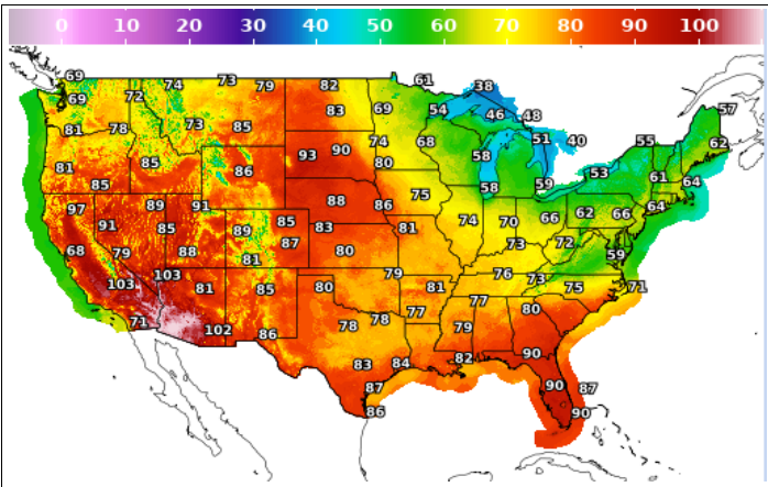
HIGH Temperature
